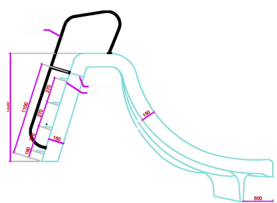
SLIDING BOARD RIGHT SIDE VIEW
