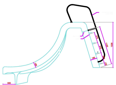
SLIDING BOARD LEFT SIDE VIEW
